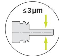
Total system runout TIR \leq 3\ \mu\text{m} at 3 \times D .
